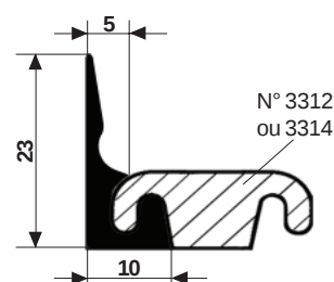
Bourrelet N°2911
